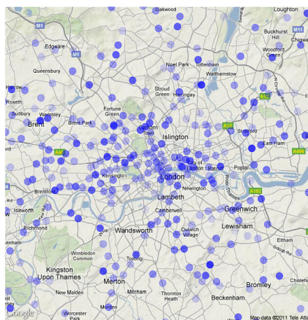
Fig. 1. The geographical distribution of IMD values, mapped using London stations: each circle is a station, darker circles have higher IMD values.
